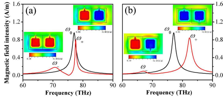
Fig. 2. The magnetic field amplitude intensity detected at the center of the resonators of a single SRR (black curve) and homo-connected SRR pair (red curve) for (a), and hetero-connected pair for (b); The insets correspond to the magnetic field maps for the split higher and lower modes, respectively.
