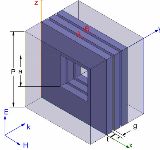
Fig. 1. Unit cell of three-metal-layer structure: the period P=600 \text{ nm} , hole size a=250 \text{ nm} , gap between layers g=20 \text{ nm} , and thickness of metal layer t is changed from 20 to 100 nm in calculations.
